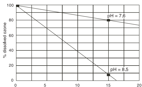
Fig. 2: Time of breakdown (mn) of dissolved ozone
